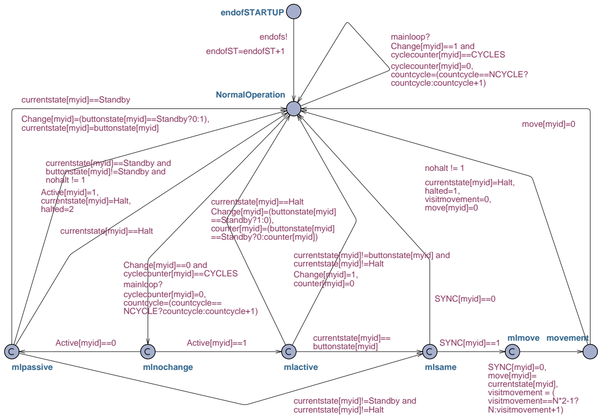
Fig. 2. Part of the automaton Station : Main loop.
