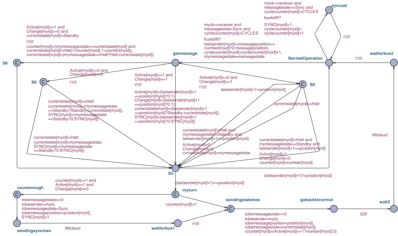
Fig. 3. Part of the automaton Station: Fast loop .
