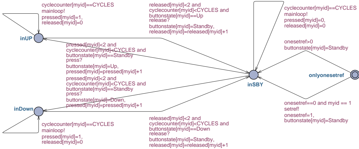
Fig. 1. The automaton Interface .
