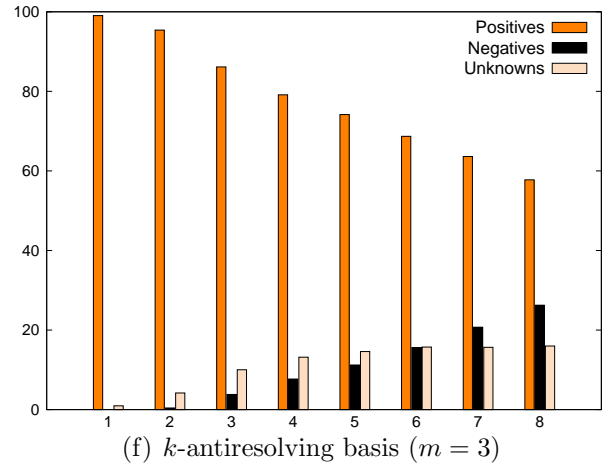
Figure 3: Six charts showing the ratio of true, false, and unknown results provided by Algorithm 1 and Algorithm 2 on different values for m \in \{1, 2, 3\} . Charts at the left are devoted to the algorithm aimed at finding a k -antiresolving set, charts at the right consider the algorithm that looks for a k -antiresolving basis.
