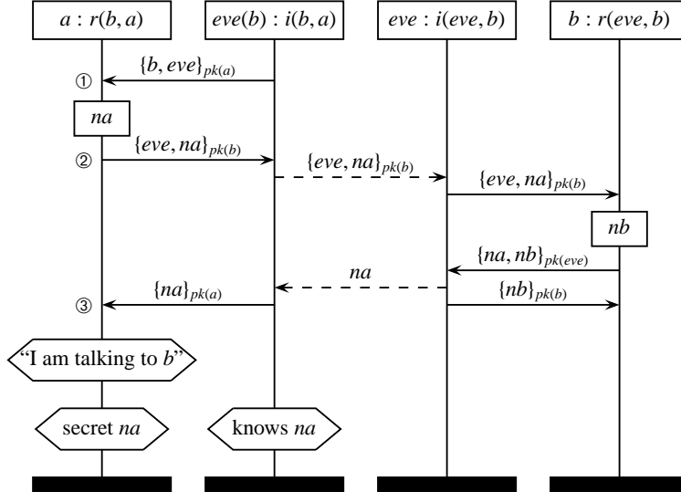
Fig. 2. Type-flaw attack on Needham-Schroeder
