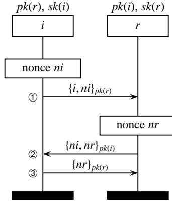
Fig. 1. Needham-Schroeder public-key authentication protocol
