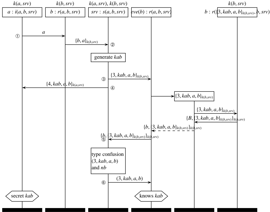
Fig. 4. Attack on key-establishment protocol
