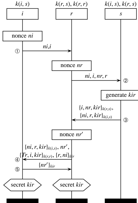
Fig. 5. Lowe modified KSL
