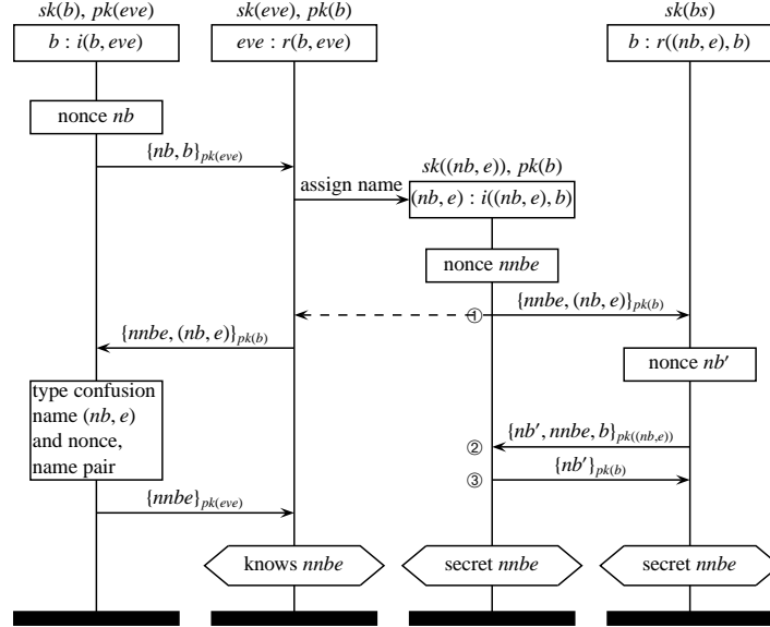
Fig. 8. Assigned-name attack
