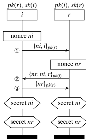
Fig. 7. A variant of NSL
