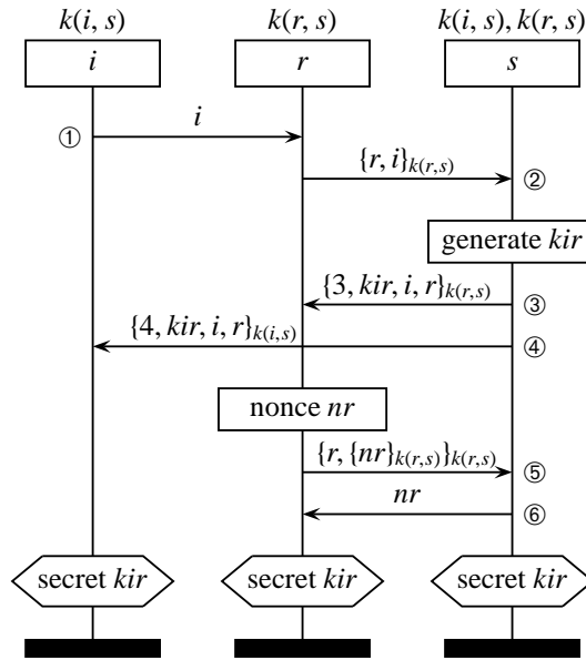
Fig. 3. Key-establishment protocol
