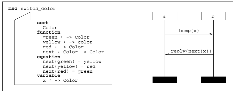
Figure 1: Combining MSC and algebraic specifications.
