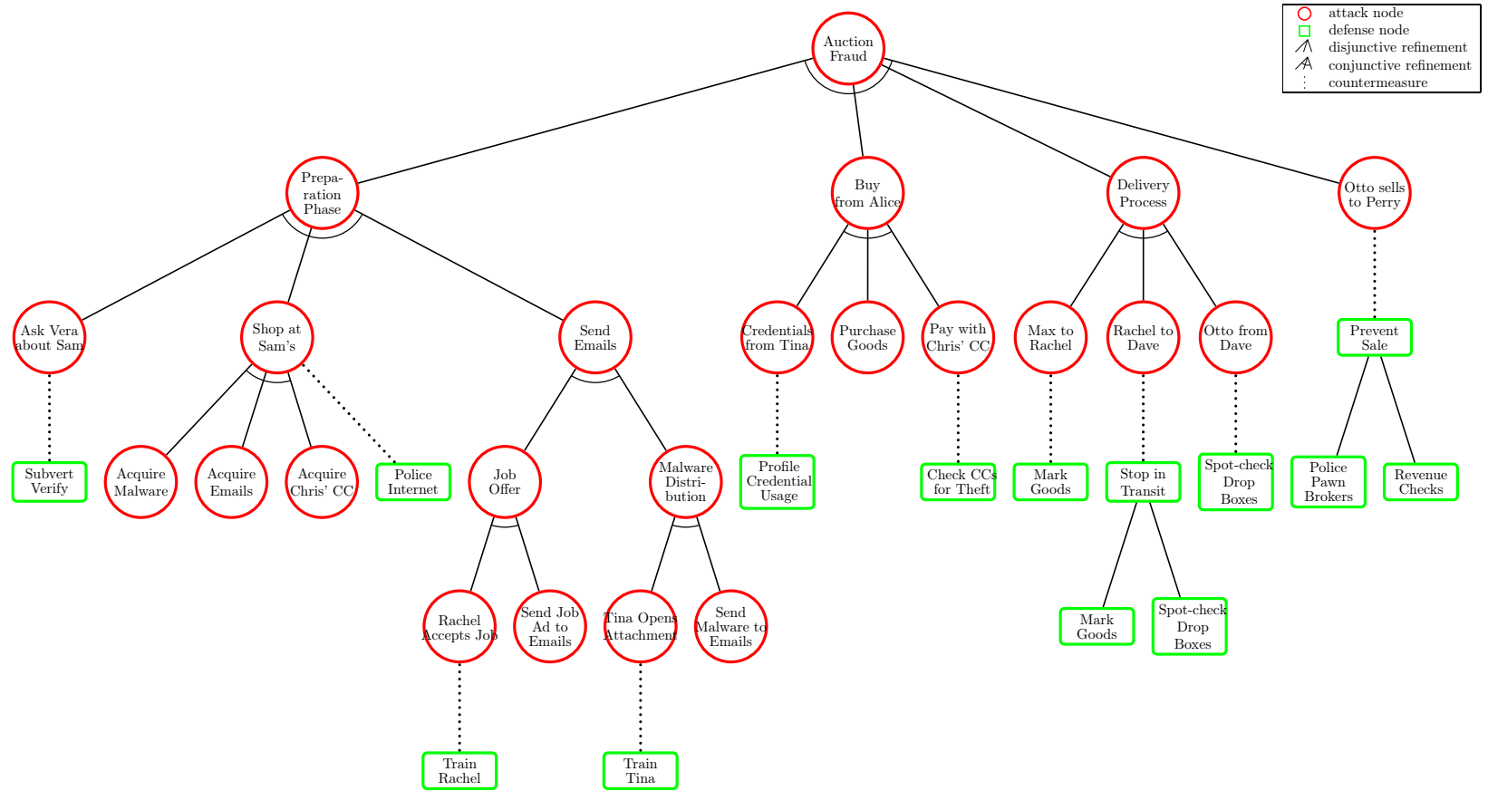
An online auction fraud scenario.
