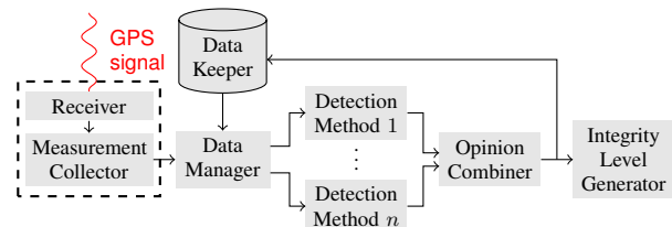
Figure 2: The components of the prototype.
